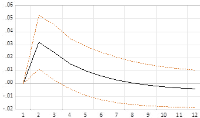
Response of LWAMAR to LPGDP Innovation using Cholesky (d.f. adjusted) Factors
